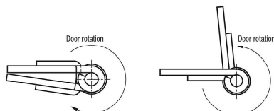
Hinges with closing spring
