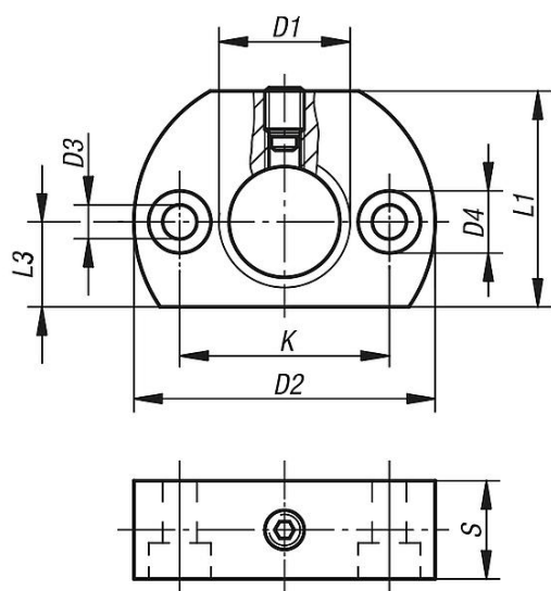
Form A fastening hole parallel to indexing plunger
