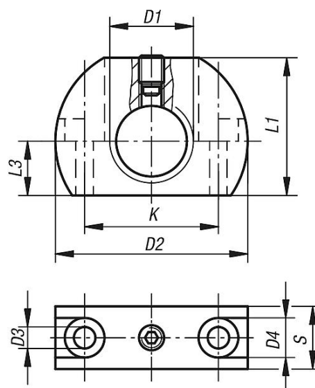
Form B fastening hole vertical to indexing plunger
